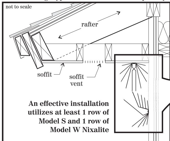
Section through typical soffit/eave - for example only
