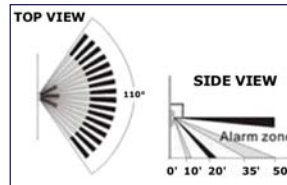
Detection zone for module is 50ft deep and 110° wide
